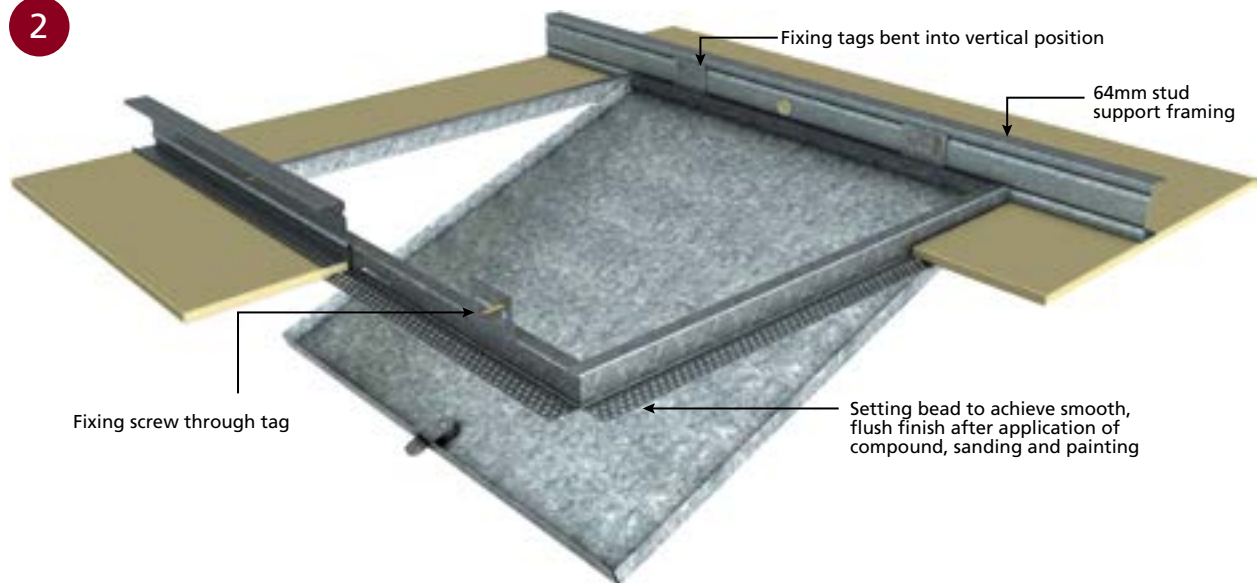
■ MFAP INSTALLATION
