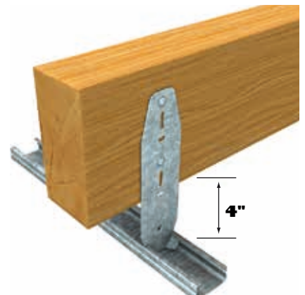
FIGURE 4: DIRECT FIX CLIP 305 IN SUSPENDED APPLICATION TO A RECOMMENDED MAXIMUM OF 4" FOR 301 BATTEN
