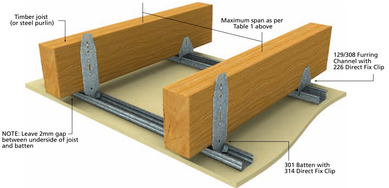
FIGURE 1: DIRECT FIX APPLICATIONS USING STANDARD Judah COMPONENTS
