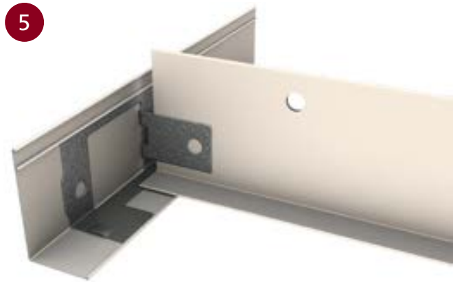
■ DUO8 WITH 705 CLIP
